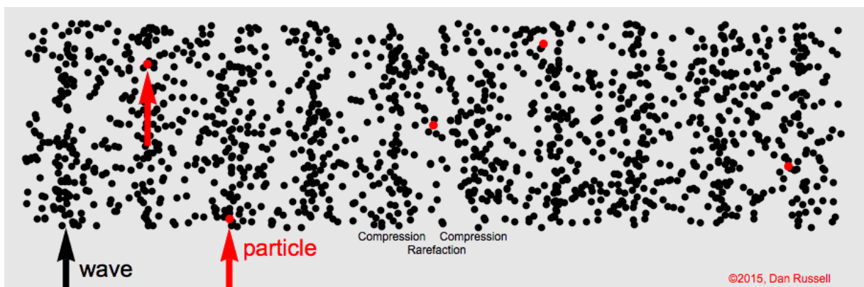
Wave and particle duality and illustration.
